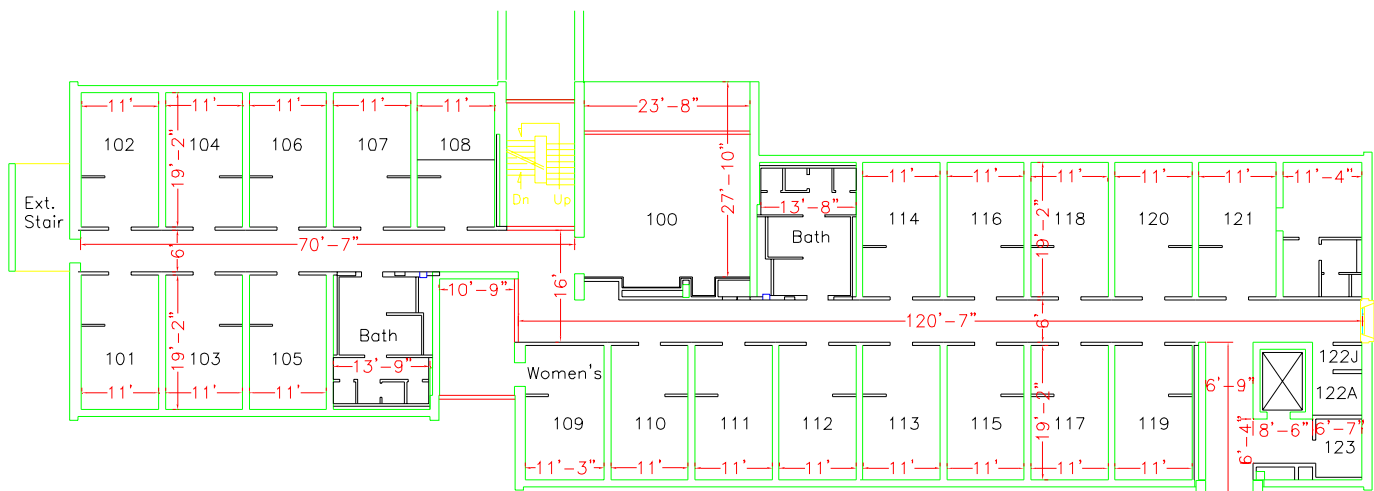
PATRICK HALL - FIRST FLOOR
